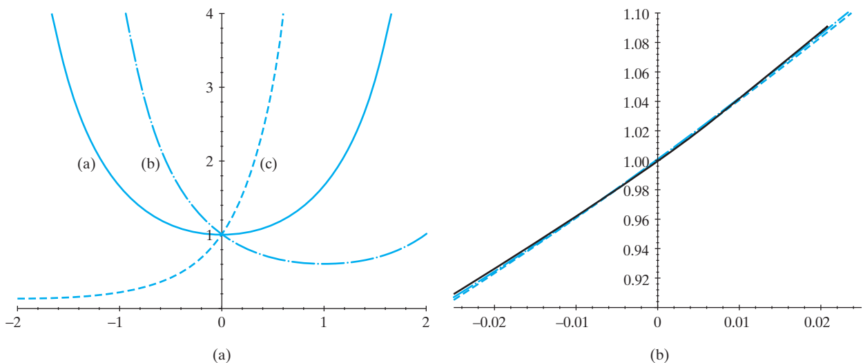
Figure 3.3-3 Moment-generating functions
